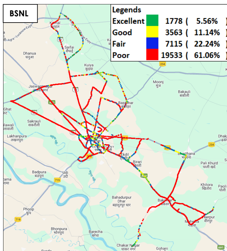
Figure-26: Signal strength 3G/2G network mode – BSNL.
