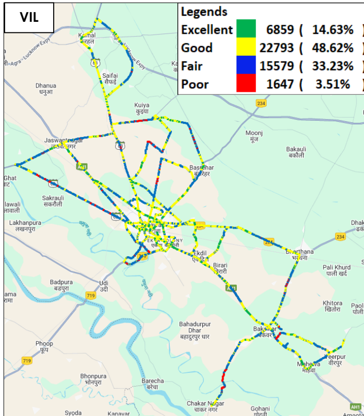
Figure-31: Signal strength auto-selection mode 5G/4G/3G/2G – VIL.
