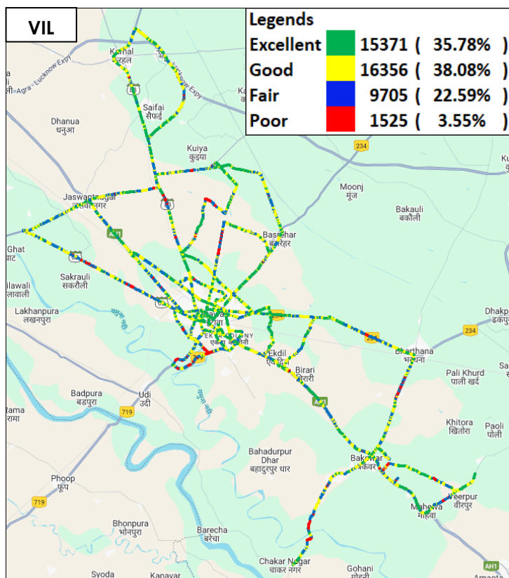
Figure-27: Signal strength 3G/2G network mode – VIL.
