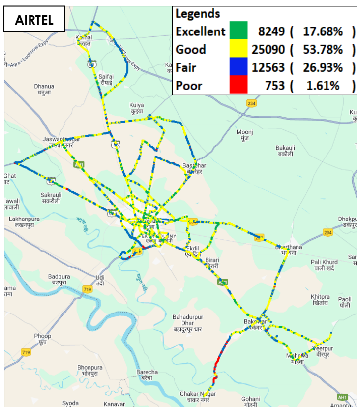
Figure-28: Signal strength auto-selection mode 5G/4G/3G/2G – AIRTEL.
