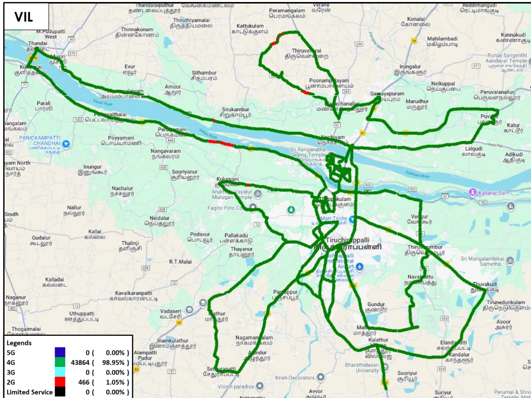
Figure-19: Serving technology plot in auto-selection mode (5G/4G/3G/2G) voice - VIL
