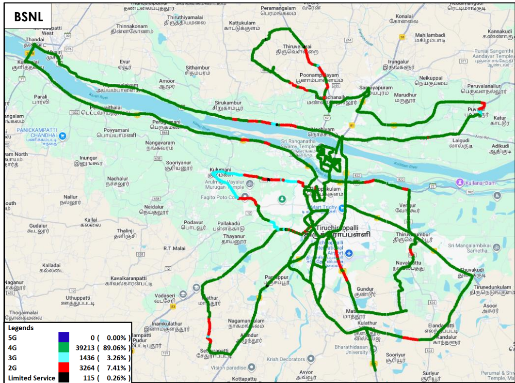
Figure-17: Serving technology plot in auto-selection mode (5G/4G/3G/2G) voice - BSNL.
