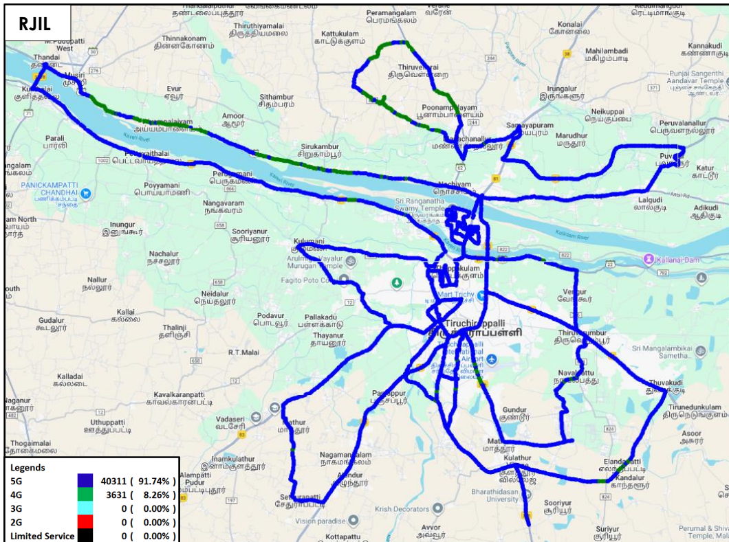
Figure-25: Serving technology plot in auto-selection mode (5G/4G/3G/2G) data - RJIL.
