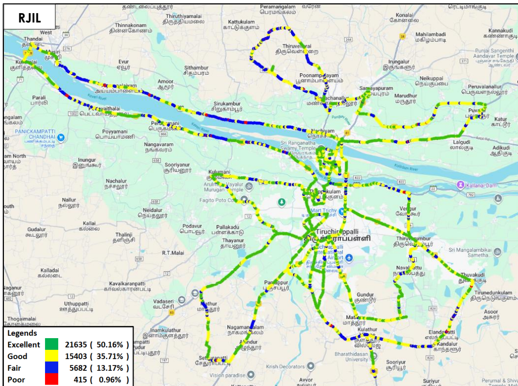
Figure-35: Signal strength auto-selection mode (5G/4G/3G/2G) voice – RJIL.
