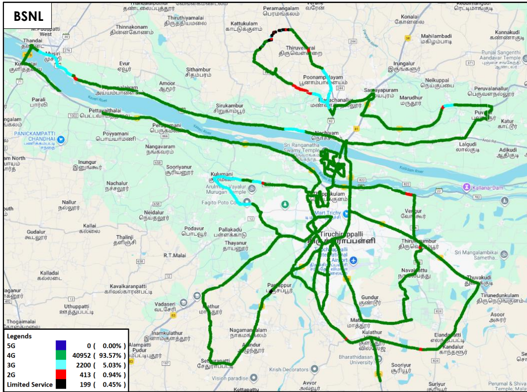
Figure-24: Serving technology plot in auto-selection mode (5G/4G/3G/2G) data - BSNL.
