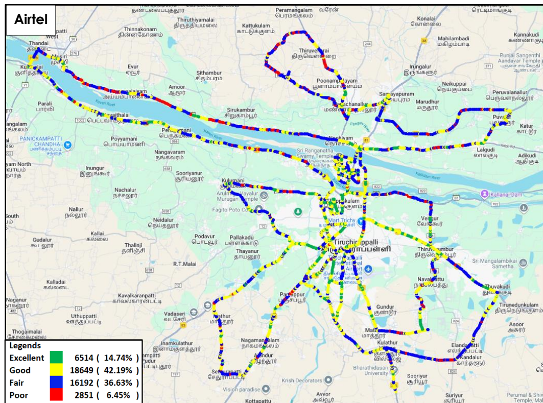
Figure-37: Signal strength auto-selection mode (5G/4G/3G/2G) data– AIRTEL.
