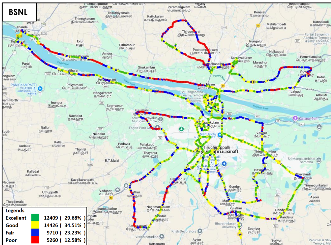
Figure-31: Signal strength 3G/2G network mode - BSNL.
