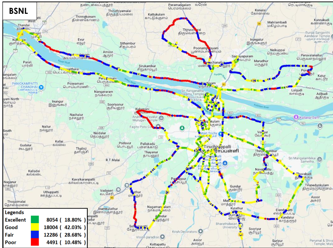
Figure-34: Signal strength auto-selection mode (5G/4G/3G/2G) voice – BSNL.
