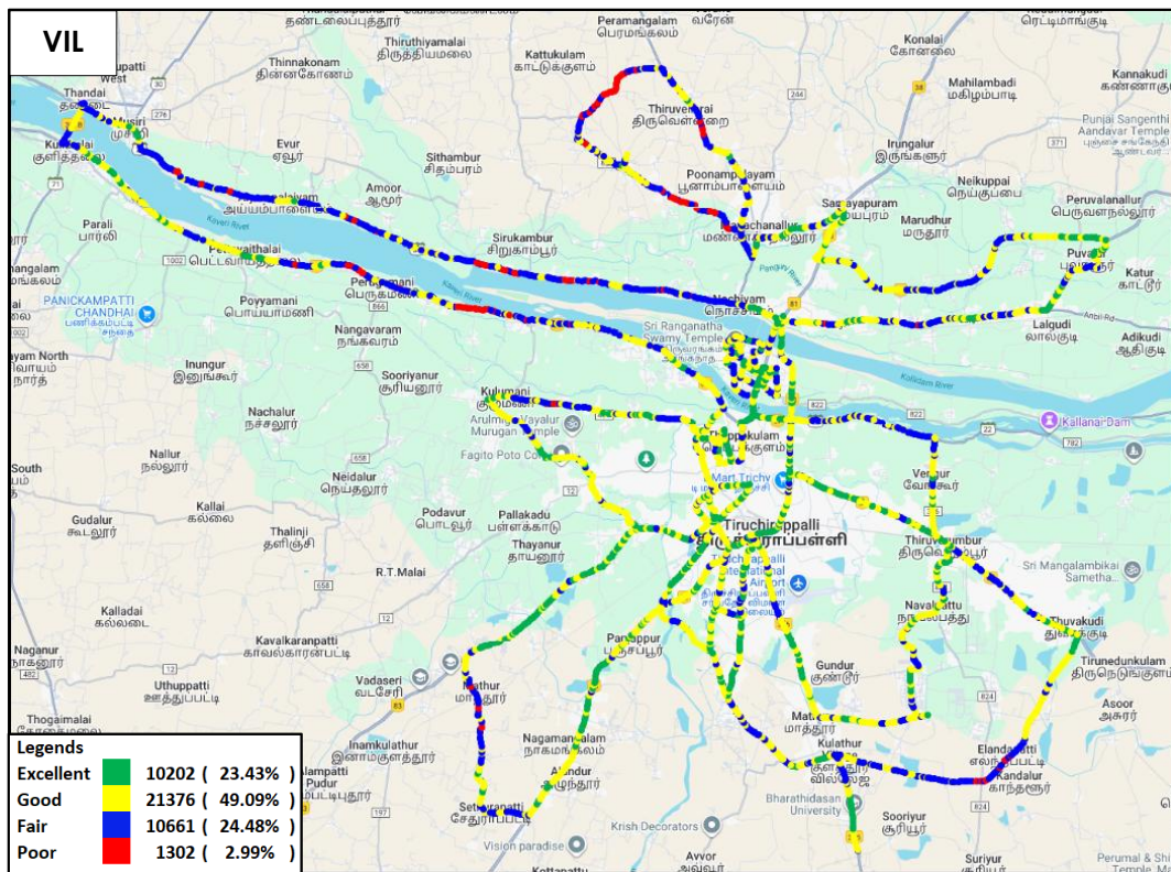
Figure-36: Signal strength auto-selection mode (5G/4G/3G/2G) voice – VIL.
