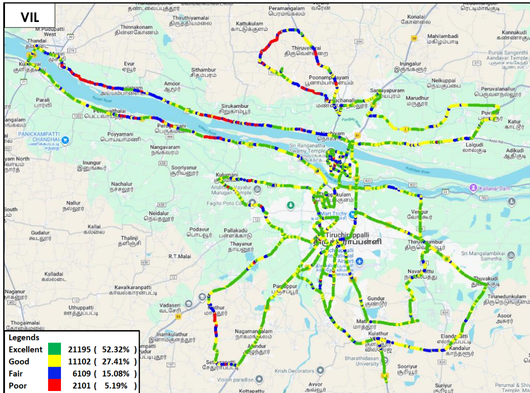
Figure-32: Signal strength 3G/2G network mode - VIL.
