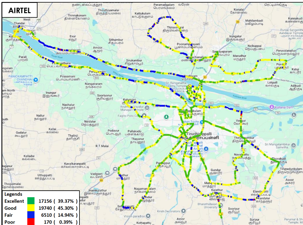
Figure-33: Signal strength auto-selection mode (5G/4G/3G/2G) voice – AIRTEL.
