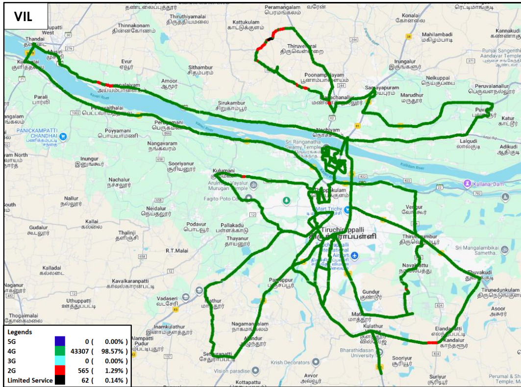
Figure-26: Serving technology plot in auto-selection mode (5G/4G/3G/2G) data - VIL
