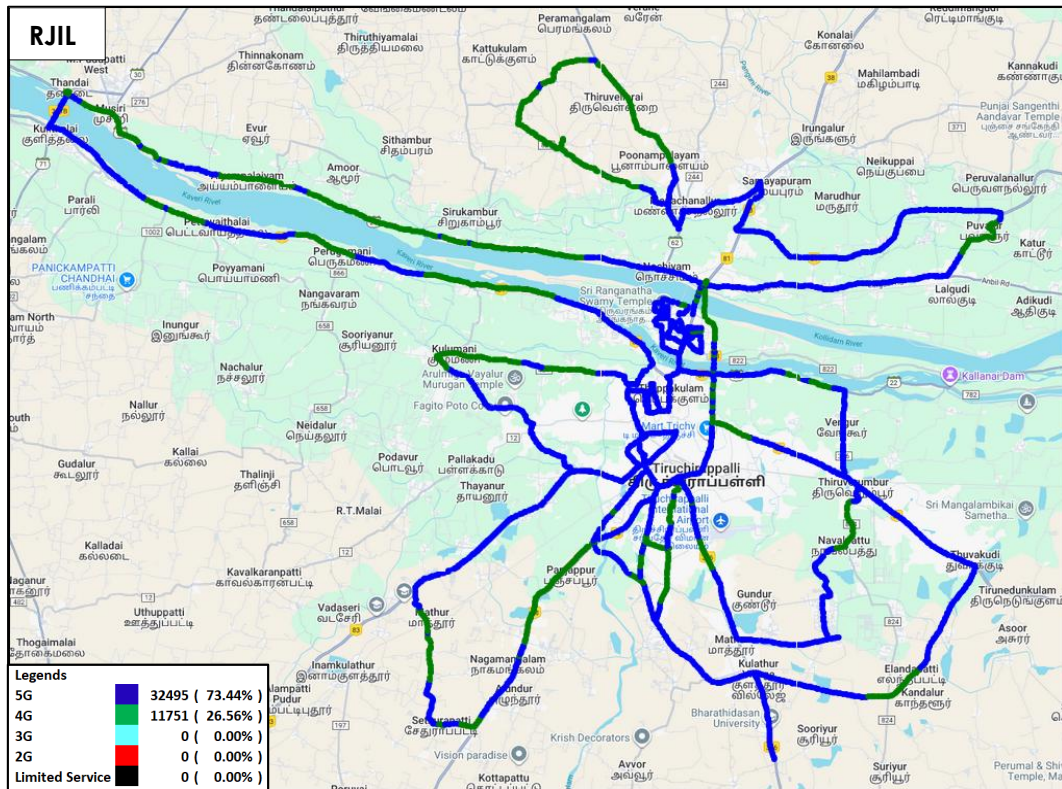
Figure-18: Serving technology plot in auto-selection mode (5G/4G/3G/2G) voice - RJIL.
