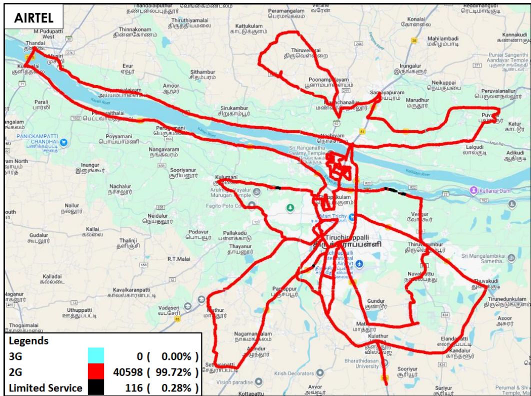
Figure-9: Serving technology plot 3G/2G network mode - AIRTEL
