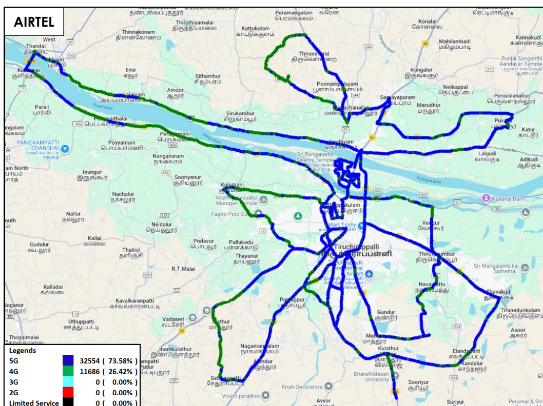
Figure-23: Serving technology plot in auto-selection mode (5G/4G/3G/2G) data - AIRTEL.
