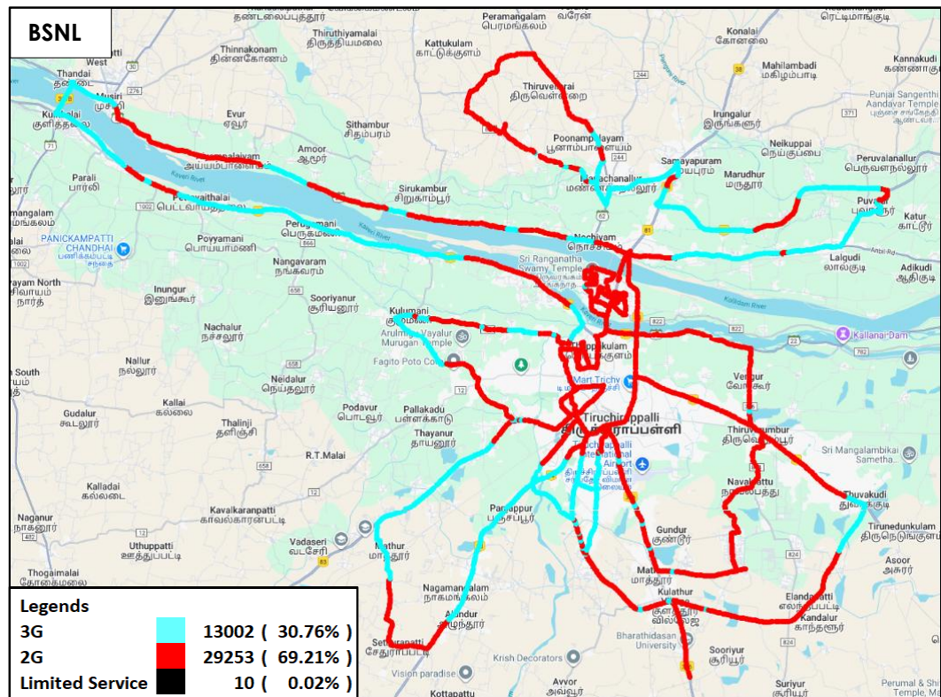
Figure-10: Serving technology plot 3G/2G network mode - BSNL.
