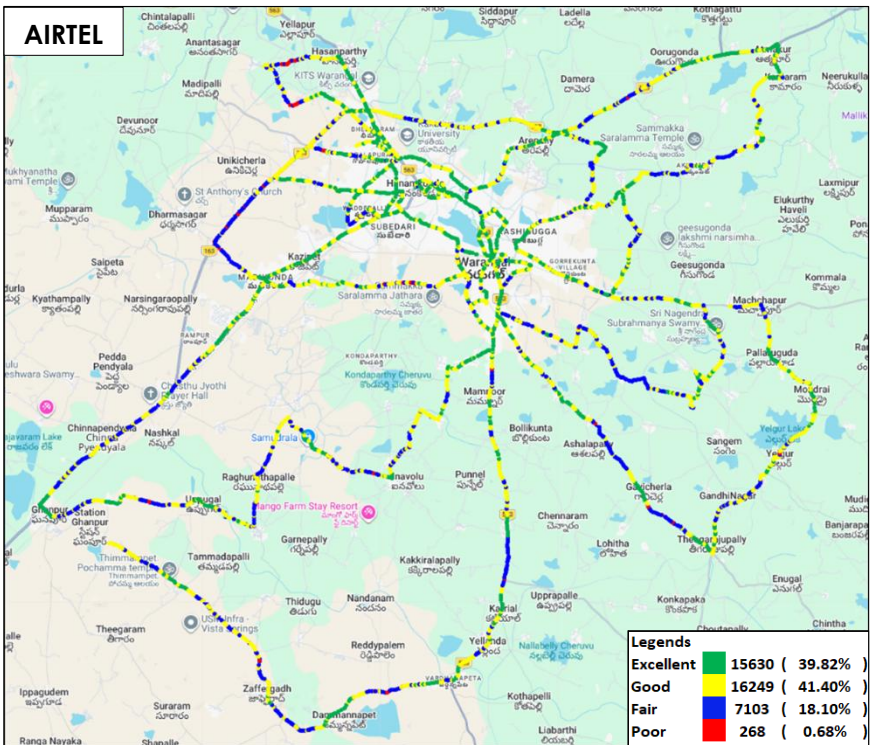
Figure-32: Signal strength auto-selection mode (5G/4G/3G/2G) voice - AIRTEL.
