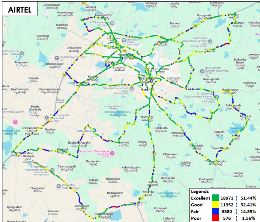
Figure-29: Signal strength 3G/2G network mode voice - AIRTEL.
