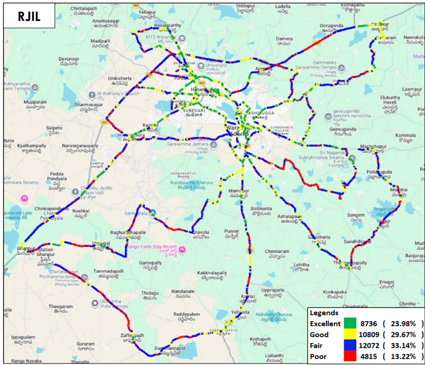
Figure-38: Signal strength auto-selection mode (5G/4G/3G/2G) data - RJIL.
