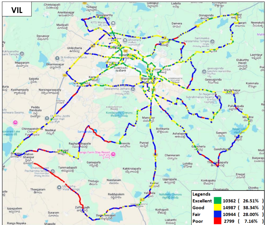
Figure-35: Signal strength auto-selection mode (5G/4G/3G/2G) voice - VIL.
