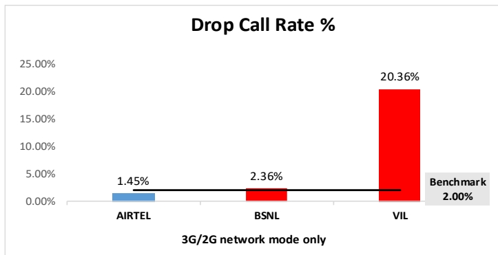
Figure-8: Performance for drop call rate.
