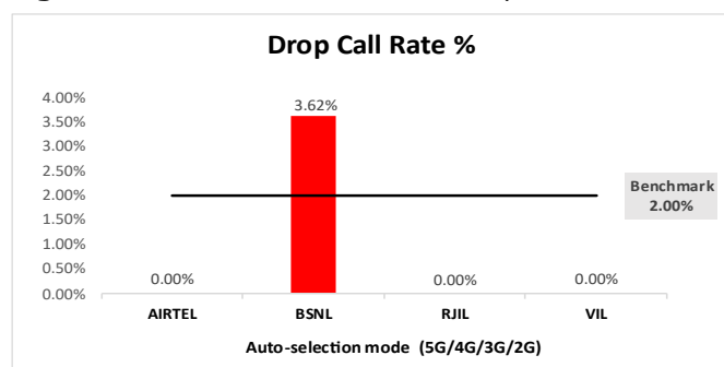
Figure-14: Performance for drop call rate.
