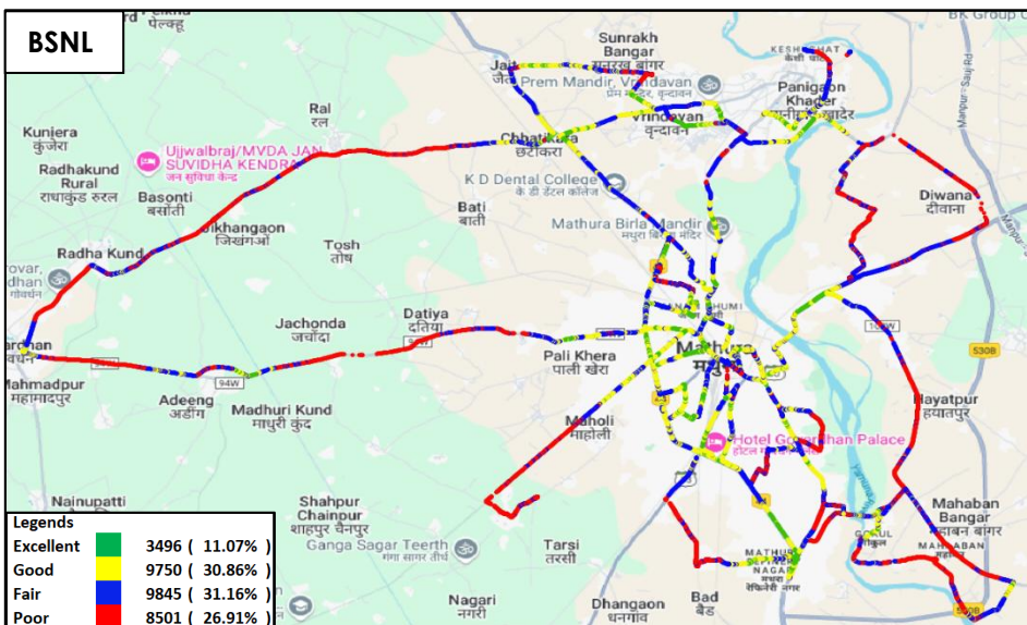
Figure-28: Signal strength auto-selection mode 5G/4G/3G/2G – BSNL.
