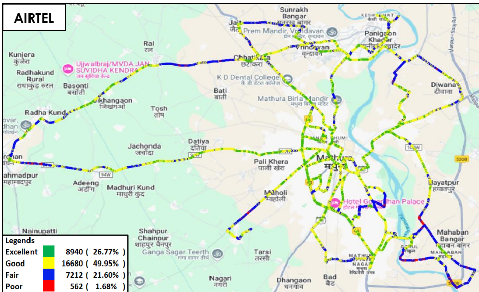
Figure-27: Signal strength auto-selection mode 5G/4G/3G/2G – AIRTEL.
