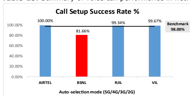
Figure-13: Performance for call setup success rate
