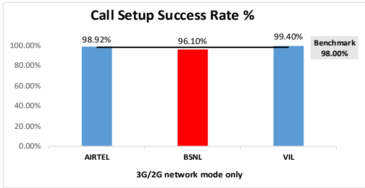
Figure-7: Performance for call setup success rate.
