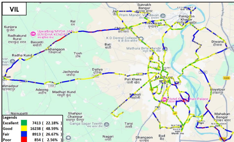
Figure-30: Signal strength auto-selection mode 5G/4G/3G/2G – VIL.
