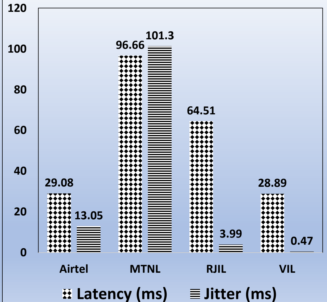
Average Latency/Jitter - Dynamic
