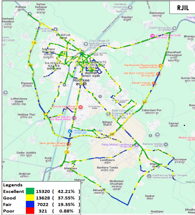
Figure-30: Signal strength auto-selection mode 5G/4G/3G/2G – RJIL.
