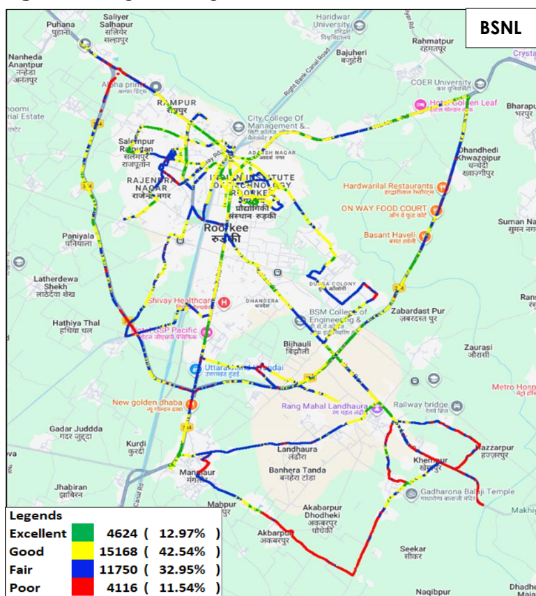
Figure-29: Signal strength auto-selection mode 5G/4G/3G/2G – BSNL.
