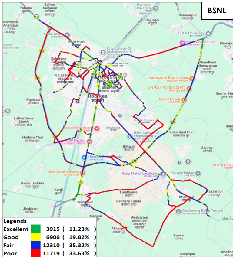
Figure-26: Signal strength 3G/2G network mode – BSNL.
