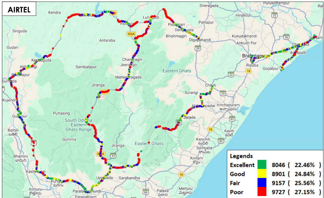
Figure-29: Signal strength 3G/2G network mode voice - AIRTEL.
