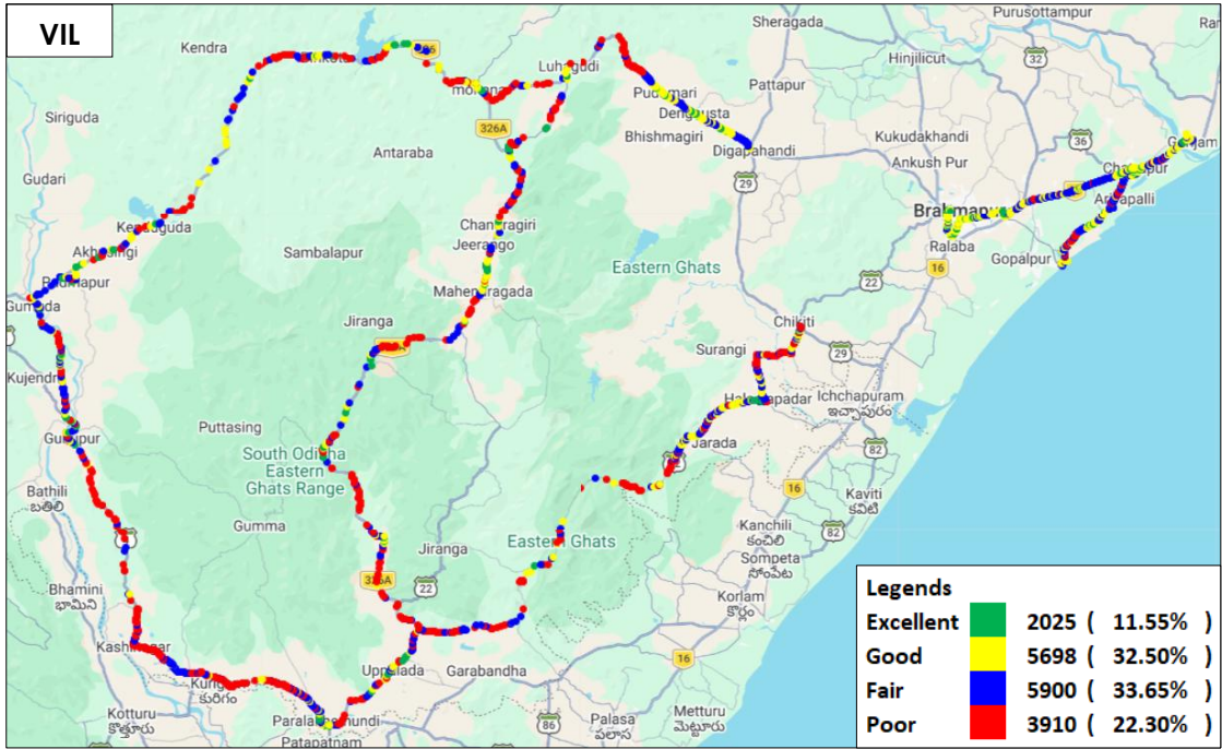
Figure-35: Signal strength auto-selection mode (5G/4G/3G/2G) voice - VIL.
