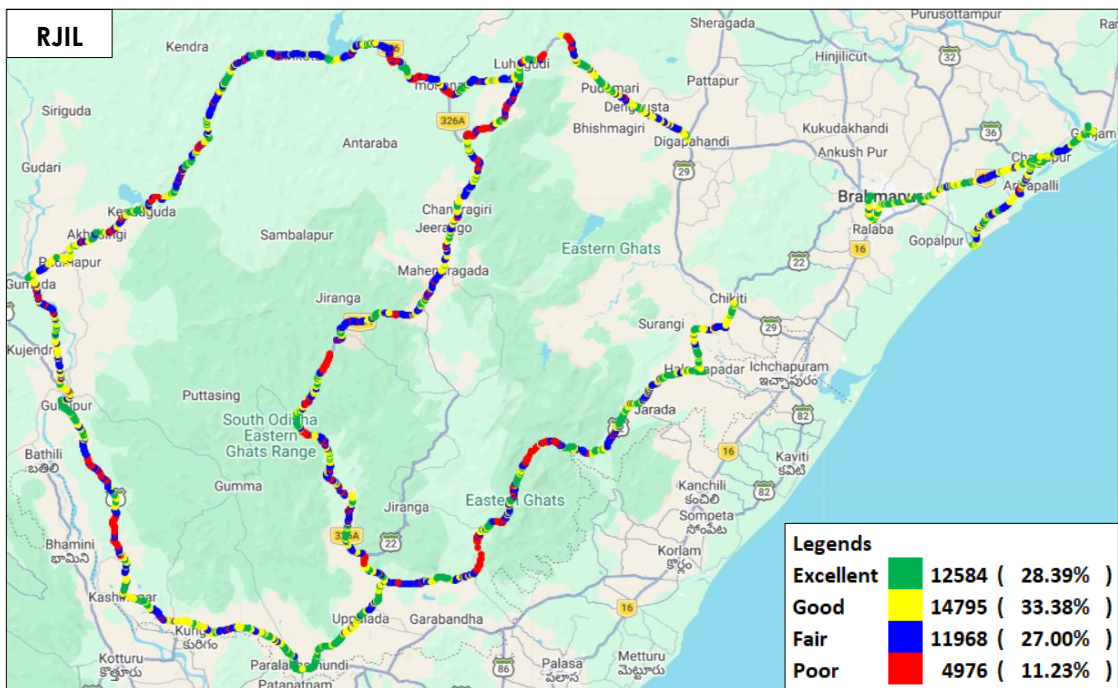
Figure-34: Signal strength auto-selection mode (5G/4G/3G/2G) voice - RJIL.
