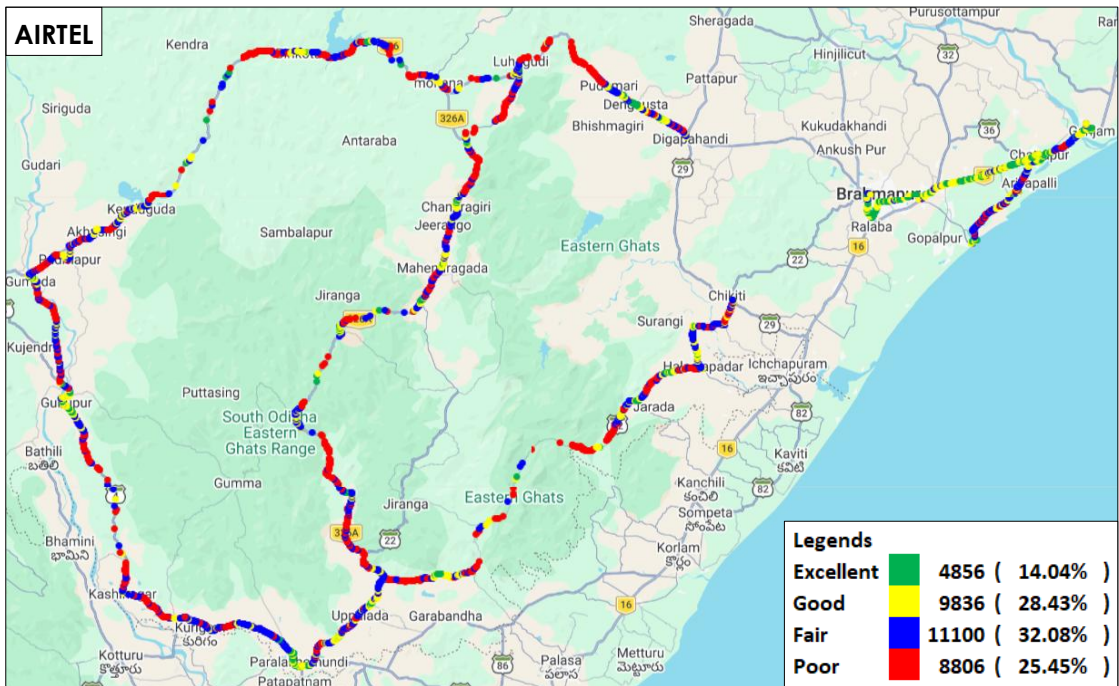
Figure-36: Signal strength auto-selection mode (5G/4G/3G/2G) data - AIRTEL.
