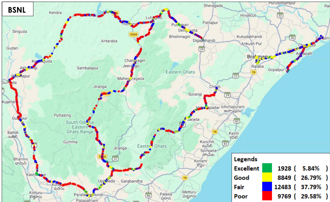
Figure-37: Signal strength auto-selection mode (5G/4G/3G/2G) data - BSNL.
