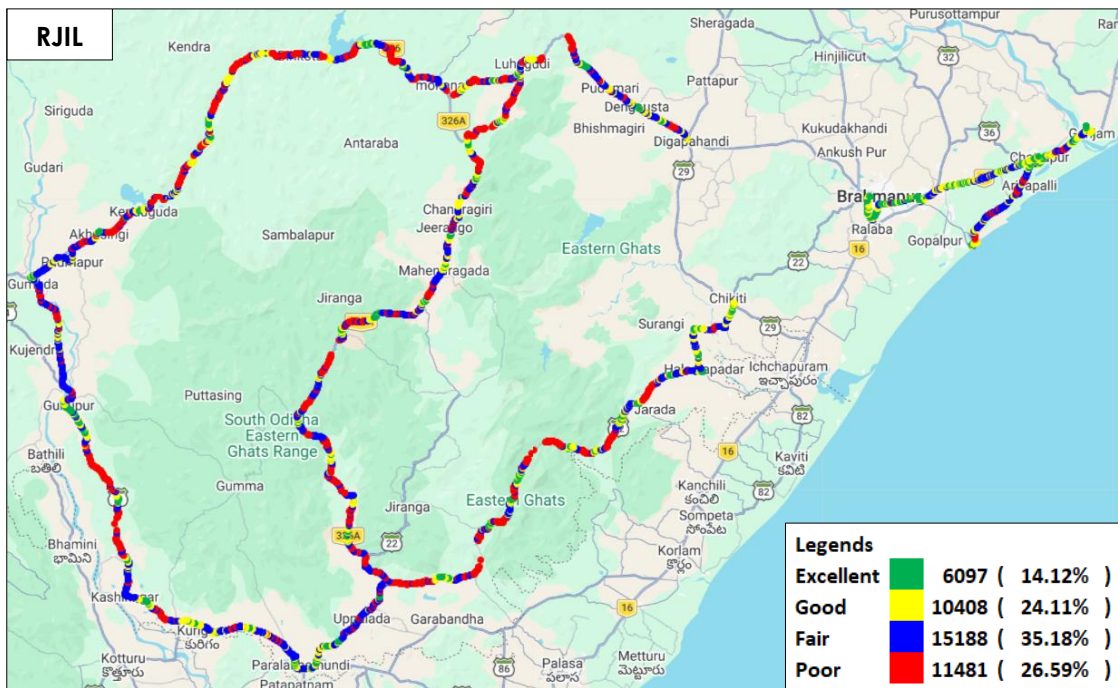
Figure-38: Signal strength auto-selection mode (5G/4G/3G/2G) data - RJIL.
