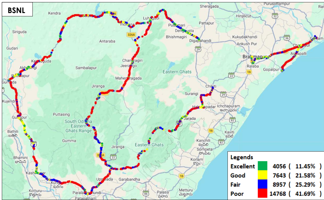
Figure-33: Signal strength auto-selection mode (5G/4G/3G/2G) voice - BSNL.
