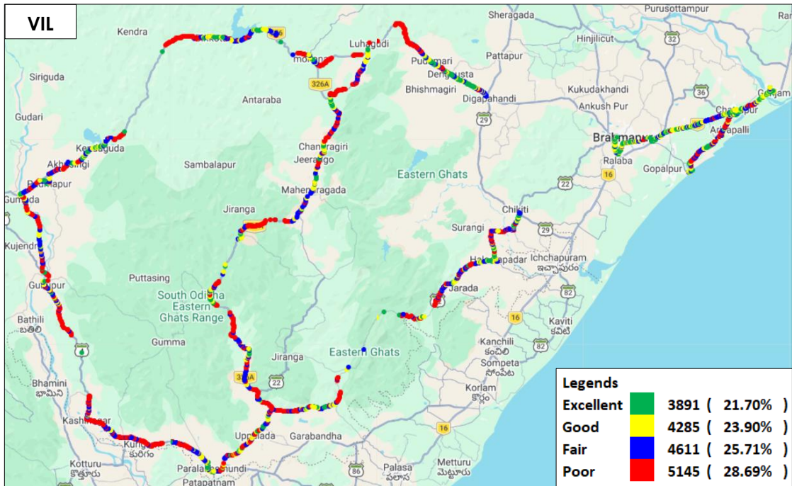
Figure-31: Signal strength 3G/2G network mode voice - VIL.
