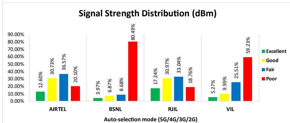
Figure-21: Signal strength distribution auto-selection mode (5G/4G/3G/2G) voice.
