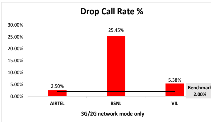
Figure-9: Performance for drop call rate.
