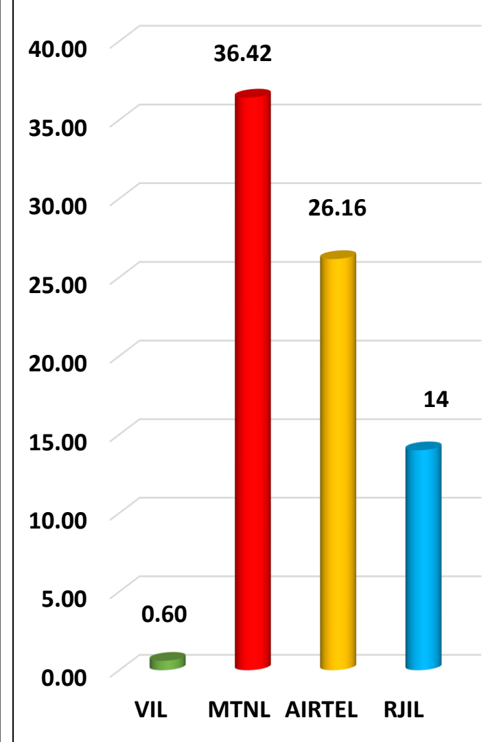
Average Jitter - Dynamic
