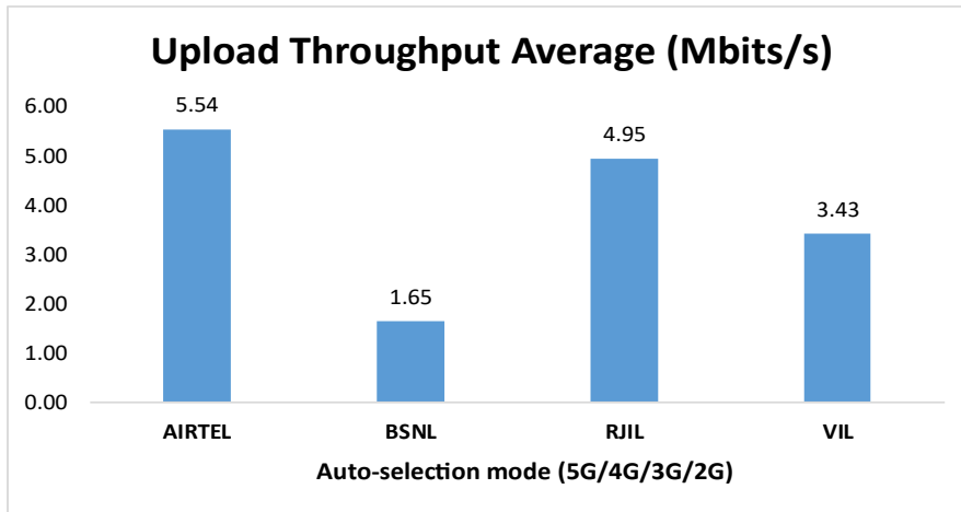
Figure-14: Upload throughput.
