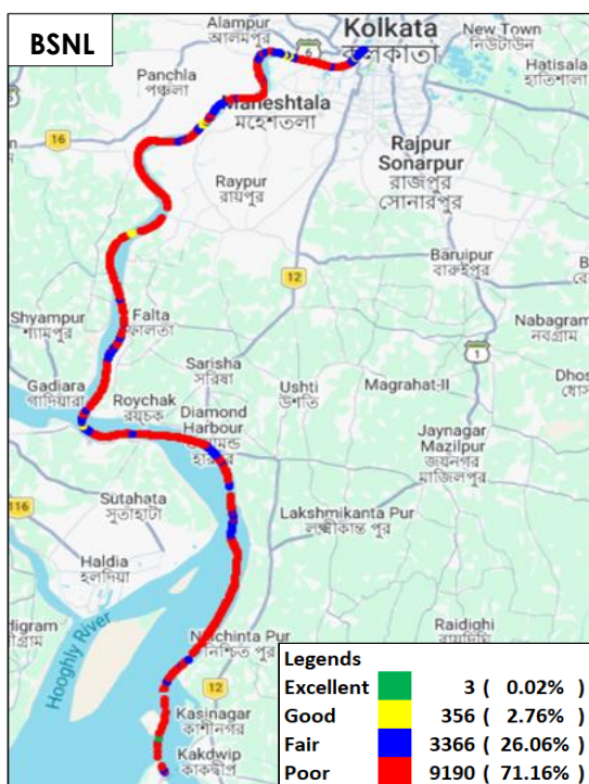
Figure-25: Signal strength auto-selection mode (5G/4G/3G/2G) data – BSNL.
