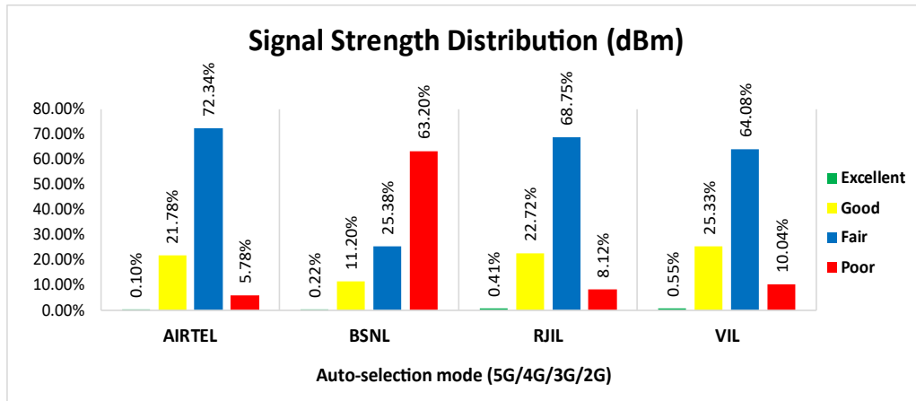
Figure-12: Signal strength distribution auto-selection mode (5G/4G/3G/2G) voice.
