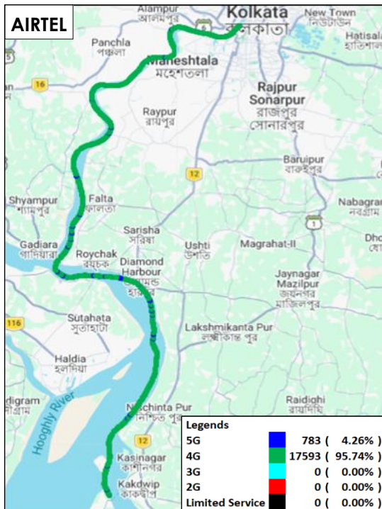
Figure-8: Serving technology plots in auto-selection mode (5G/4G/3G/2G) voice - AIRTEL.
