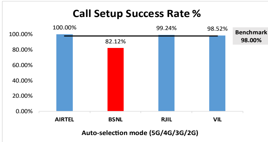
Figure-6: Performance for call setup success rate.
