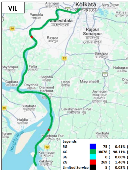
Figure-11: Serving technology plots in auto-selection mode (5G/4G/3G/2G) voice - VIL.
