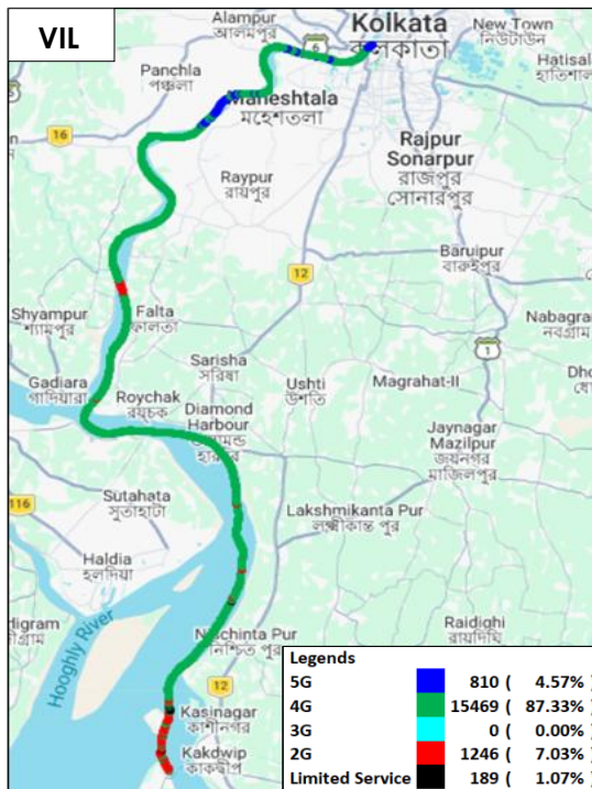
Figure-18: Serving technology plots in auto-selection mode (5G/4G/3G/2G) data - VIL.
