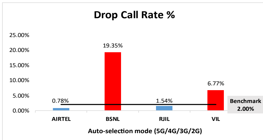
Figure-7: Performance for drop call rate.
