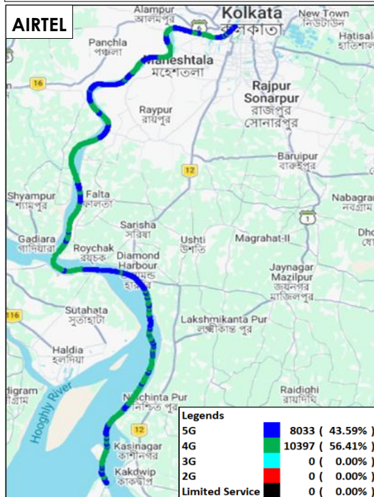
Figure-15: Serving technology plots in auto-selection mode (5G/4G/3G/2G) data - AIRTEL.
