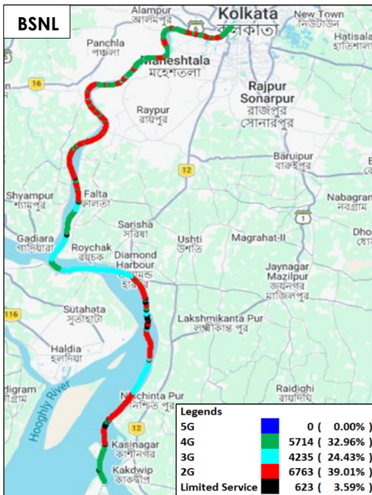
Figure-9: Serving technology plots in auto-selection mode (5G/4G/3G/2G) voice - BSNL.
