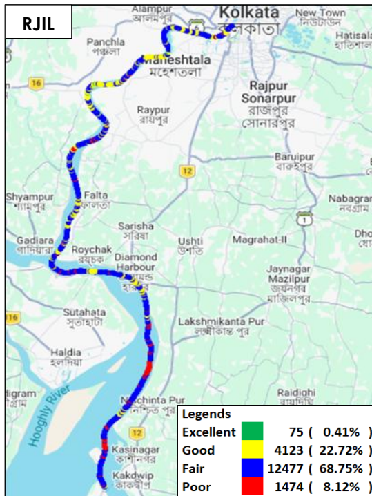
Figure-22: Signal strength auto-selection mode (5G/4G/3G/2G) voice - RJIL.
