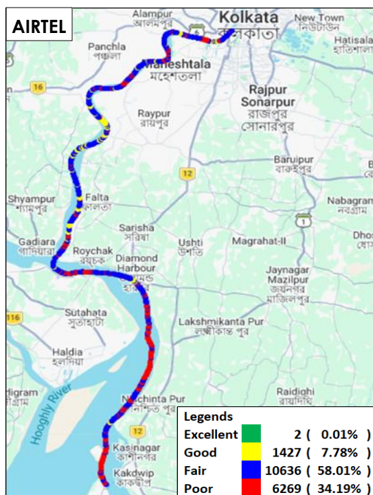
Figure-24: Signal strength auto-selection mode (5G/4G/3G/2G) data – AIRTEL.
