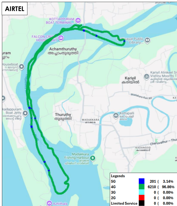
Figure-33: Serving technology plots in auto-selection mode (5G/4G/3G/2G) voice – AIRTEL.
