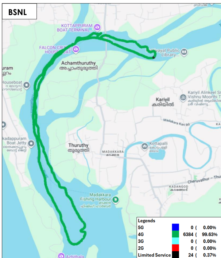
Figure-34: Serving technology plots in auto-selection mode (5G/4G/3G/2G) voice - BSNL.
