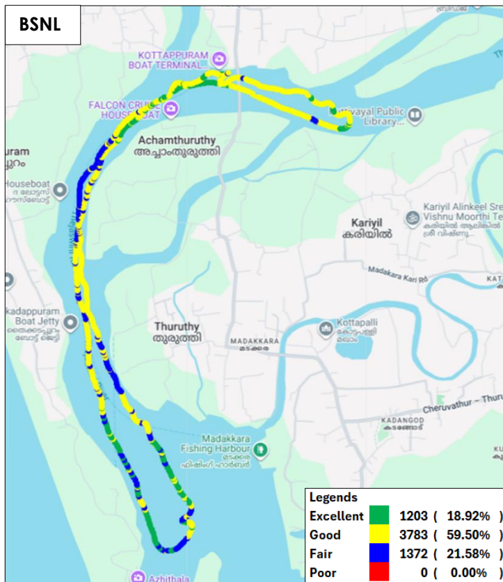
Figure-61: Signal strength auto-selection mode (5G/4G/3G/2G) data - BSNL.
