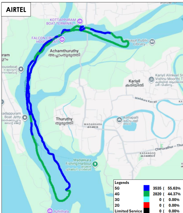
Figure-40: Serving technology plot in auto-selection mode (5G/4G/3G/2G) data - AIRTEL.
