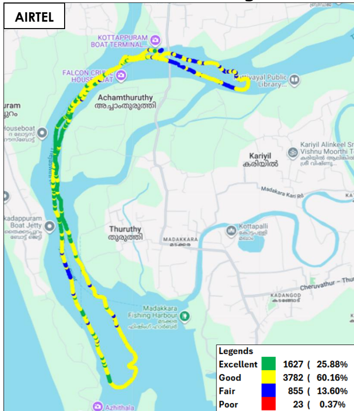
Figure-56: Signal strength auto-selection mode (5G/4G/3G/2G) voice - AIRTEL.
