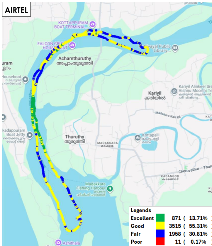
Figure-60: Signal strength auto-selection mode (5G/4G/3G/2G) data - AIRTEL.
