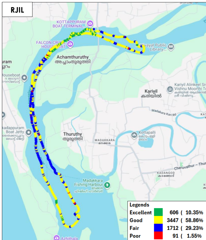
Figure-58: Signal strength auto-selection mode (5G/4G/3G/2G) voice - RJIL.
