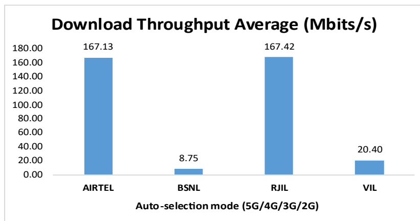
Figure 38: Download throughput.
