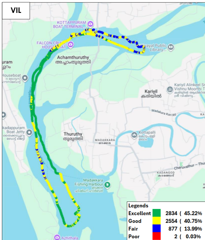
Figure-59: Signal strength auto-selection mode (5G/4G/3G/2G) voice - VIL.
