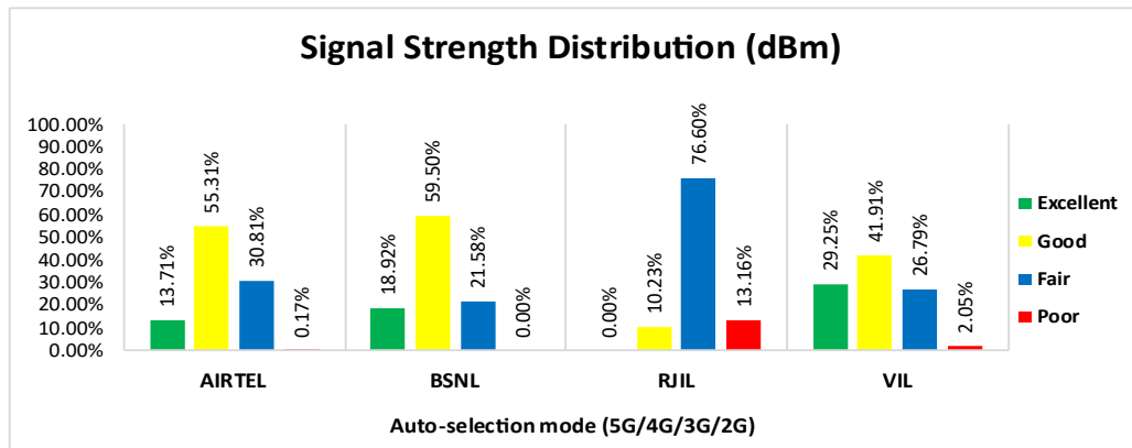
Figure-44: Signal strength distribution auto-selection mode (5G/4G/3G/2G) data.
