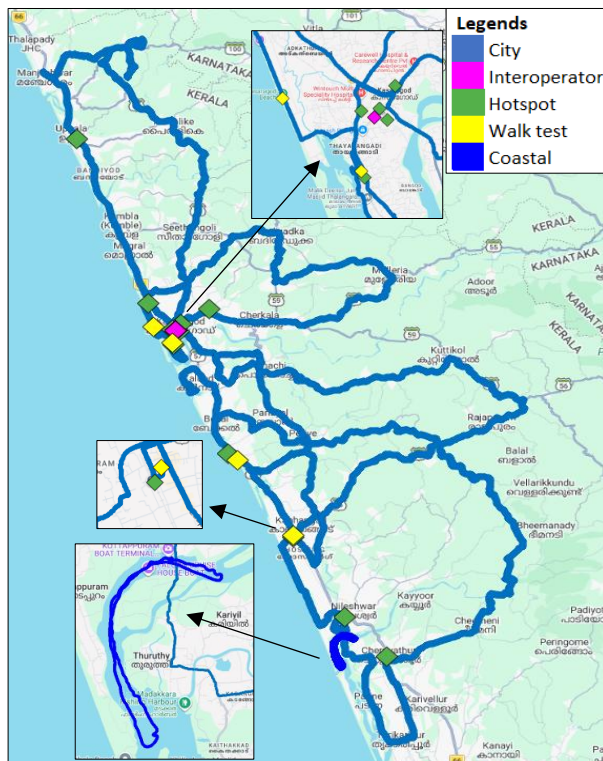
Figure-1: Drive test routes.
