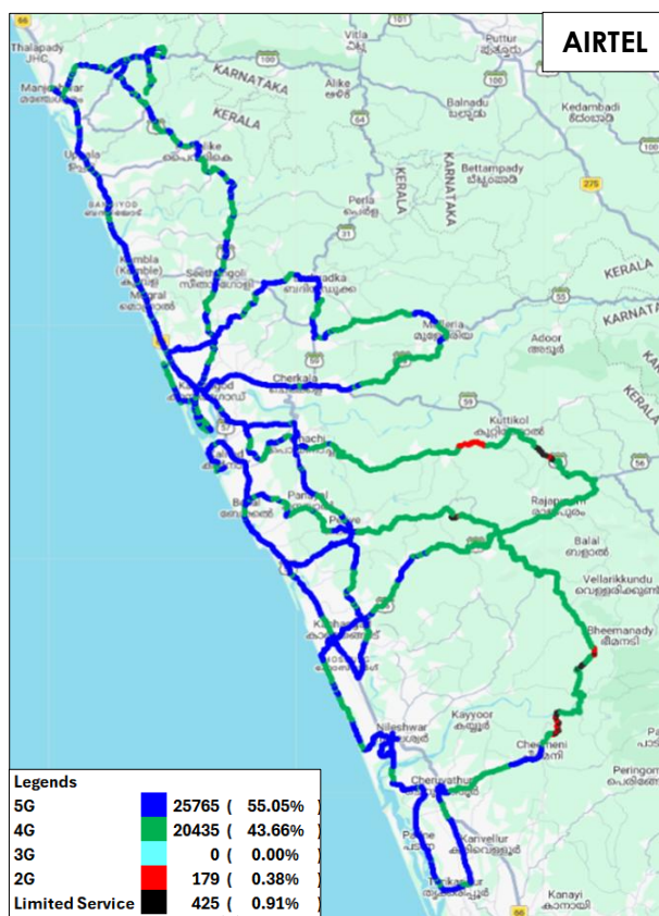
Figure-23: Serving technology plots in auto-selection mode (5G/4G/3G/2G) data - AIRTEL.
