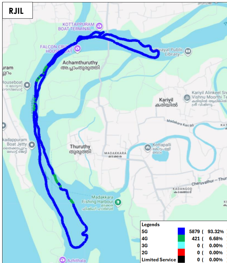
Figure-42: Serving technology plot in auto-selection mode (5G/4G/3G/2G) data - RJIL.
