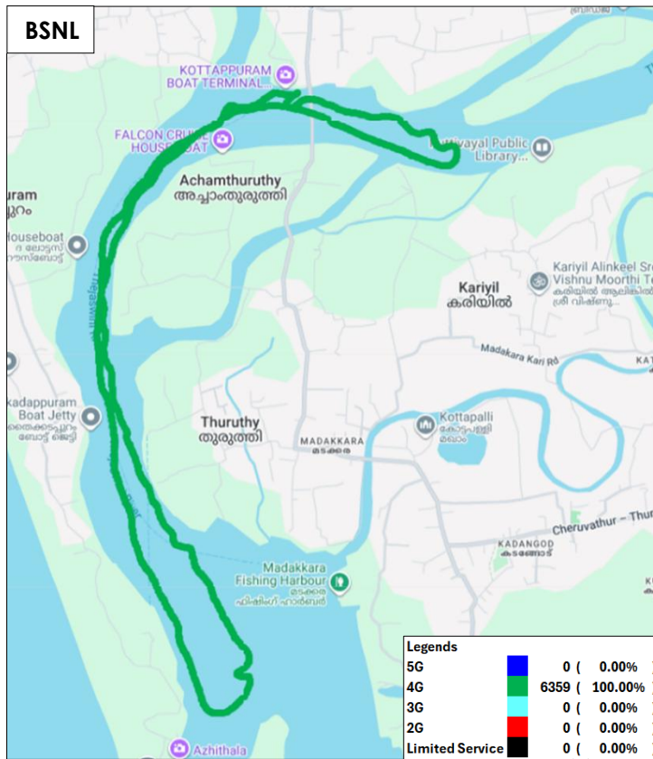
Figure-41: Serving technology plot in auto-selection mode (5G/4G/3G/2G) data - BSNL.
