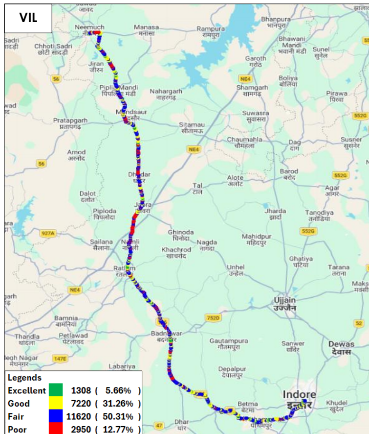
Figure-73: Signal strength auto-selection mode (5G/4G/3G/2G) data - VIL.
