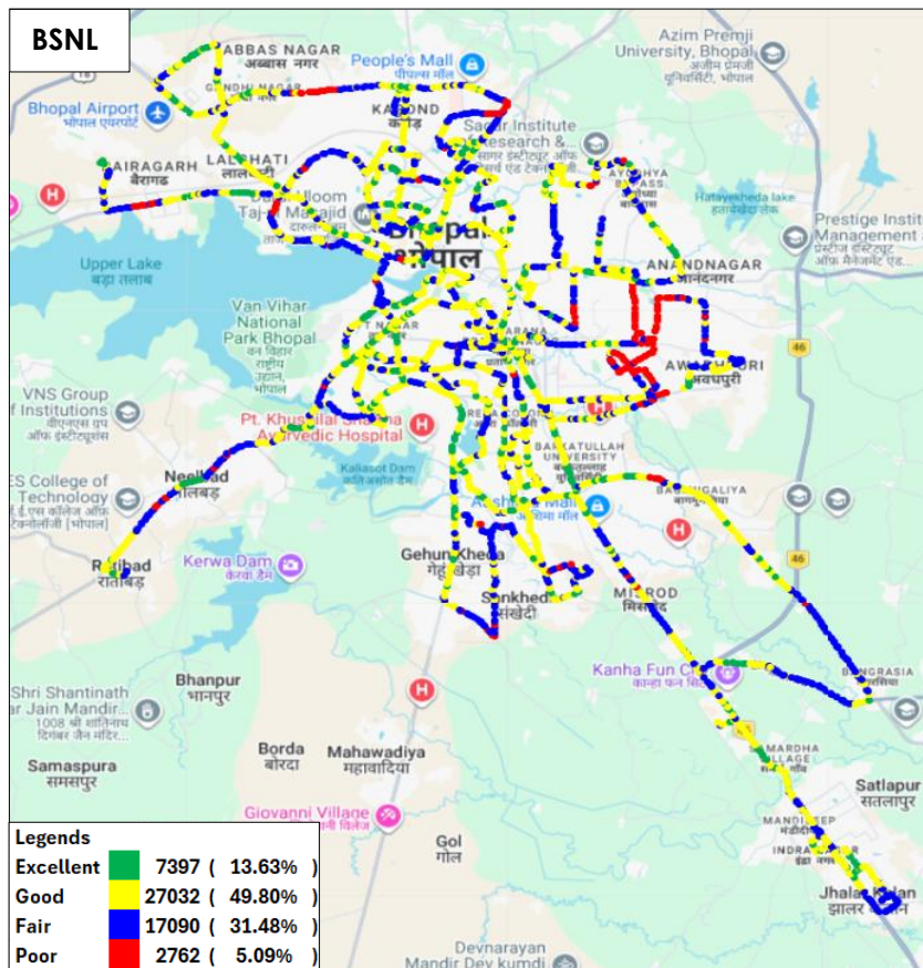
Figure-60: Signal strength auto-selection mode (5G/4G/3G/2G) data - BSNL.
