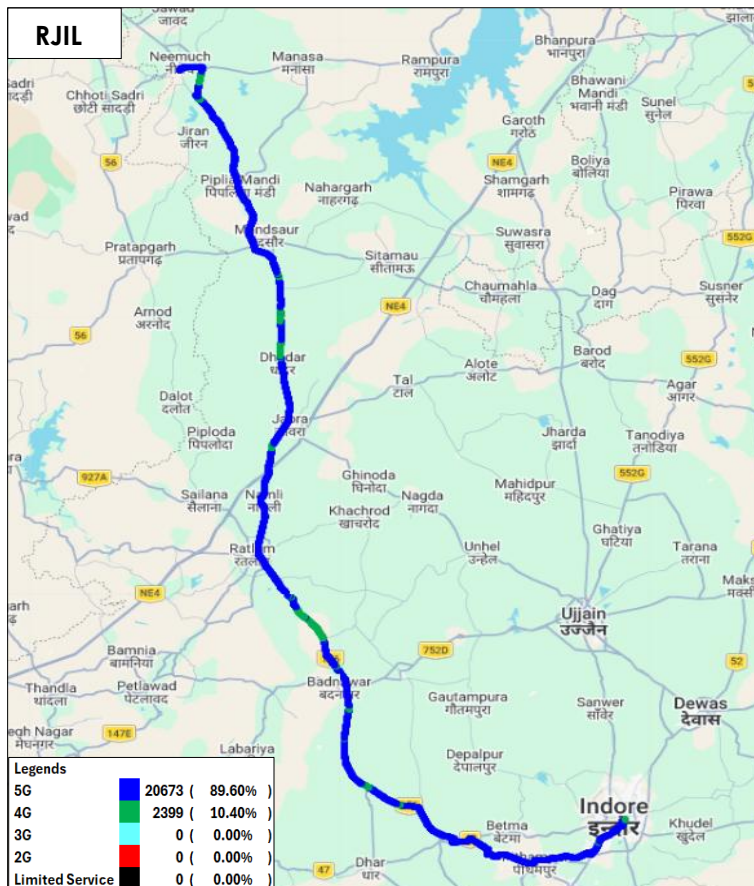
Figure-49: Serving technology plots in auto-selection mode (5G/4G/3G/2G) data - RJIL.
