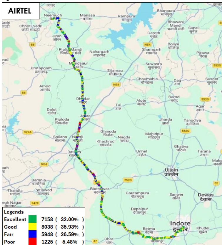
Figure-63: Signal strength 3G/2G network mode voice - AIRTEL.
