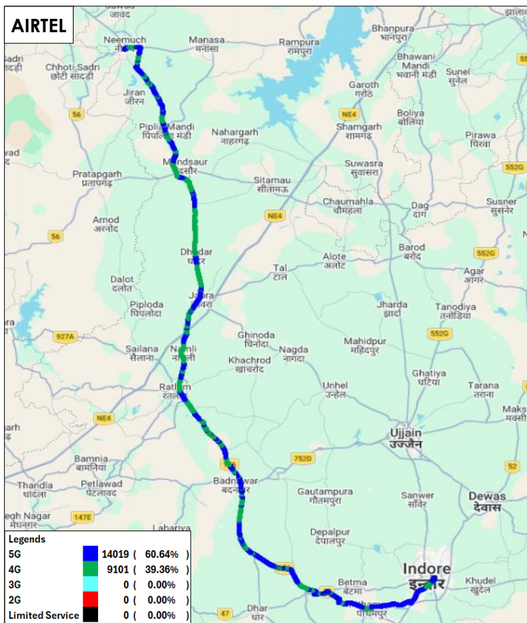
Figure-47: Serving technology plots in auto-selection mode (5G/4G/3G/2G) data - AIRTEL
