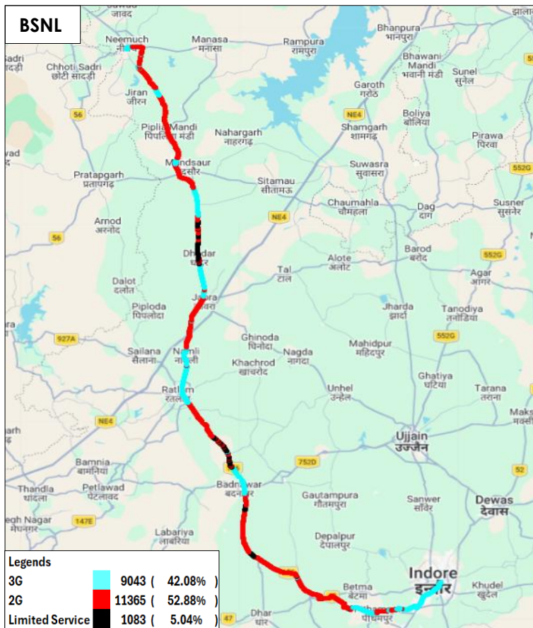
Figure-34: Serving technology plots 3G/2G network mode - BSNL.
