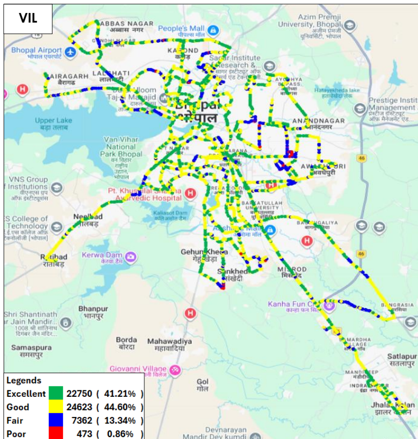
Figure-58: Signal strength auto-selection mode (5G/4G/3G/2G) voice - VIL.
