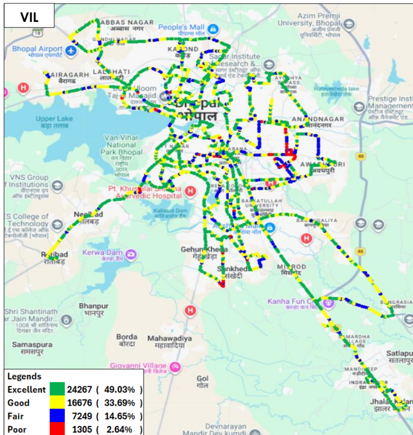
Figure-54: Signal strength 3G/2G network mode voice - VIL.
