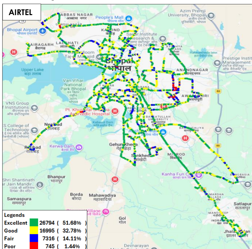
Figure-52: Signal strength 3G/2G network mode voice - AIRTEL.
