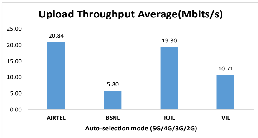
Figure-46: Upload throughput.
