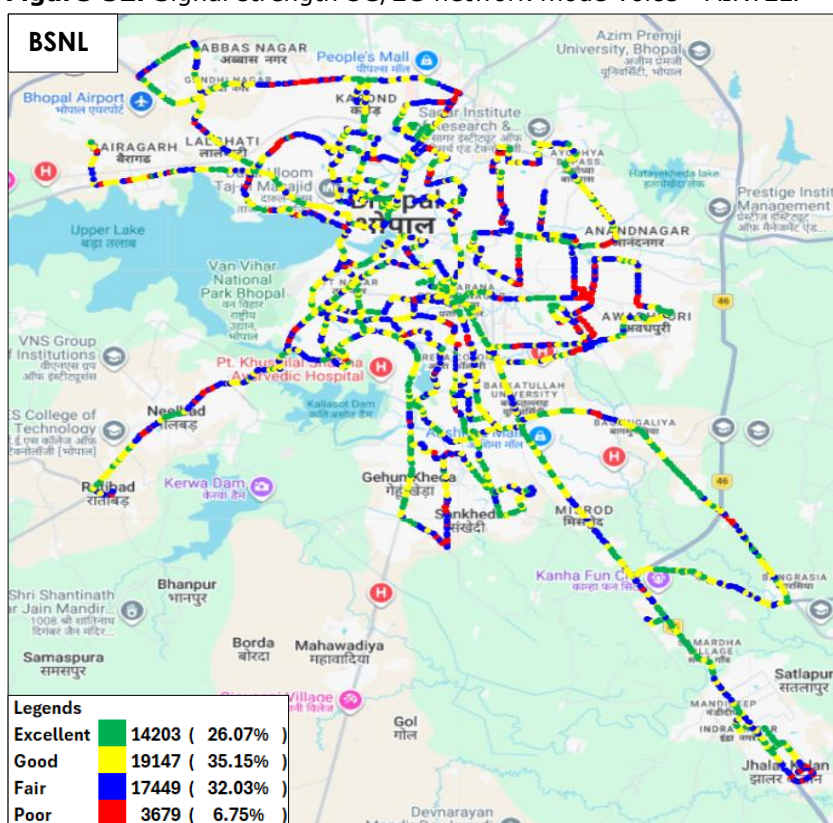
Figure-53: Signal strength 3G/2G network mode voice - BSNL.
