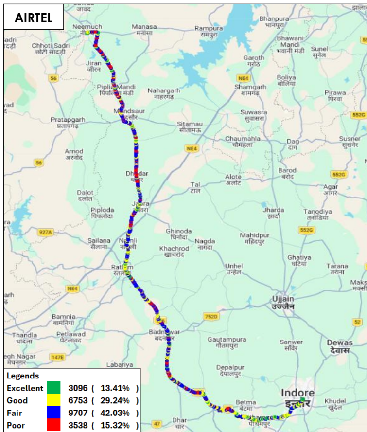
Figure-70: Signal strength auto-selection mode (5G/4G/3G/2G) data - AIRTEL.
