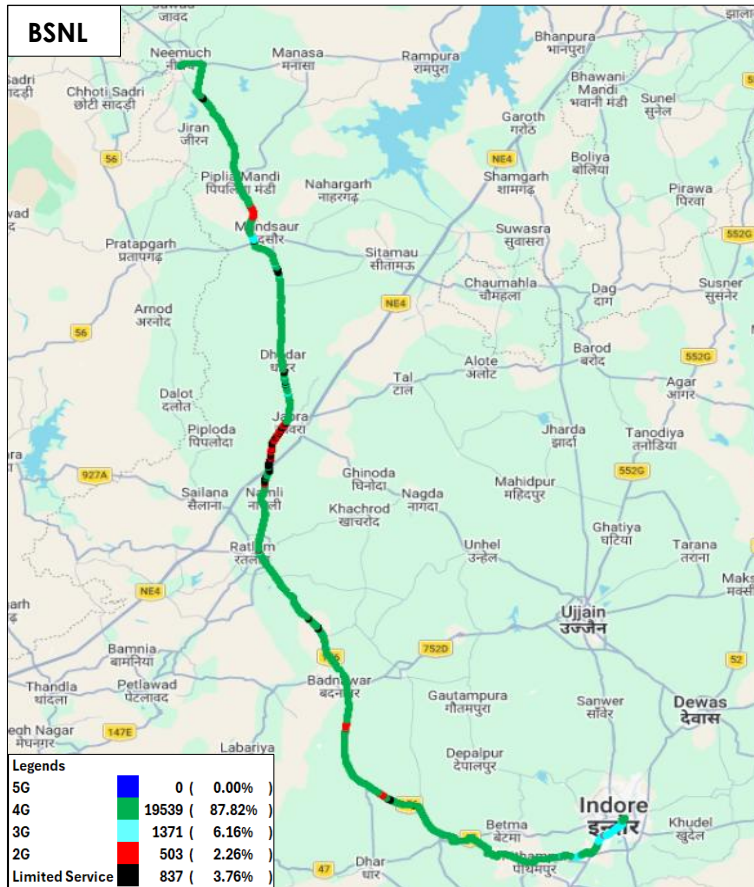
Figure-48: Serving technology plots in auto-selection mode (5G/4G/3G/2G) data - BSNL.
