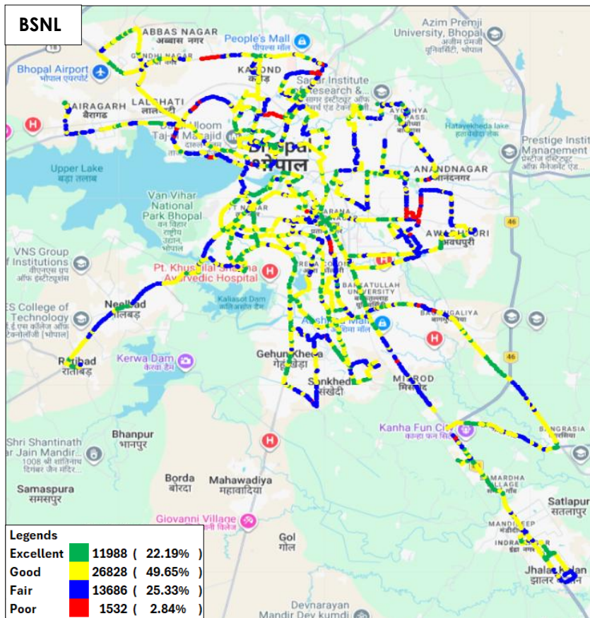
Figure-56: Signal strength auto-selection mode (5G/4G/3G/2G) voice - BSNL.
