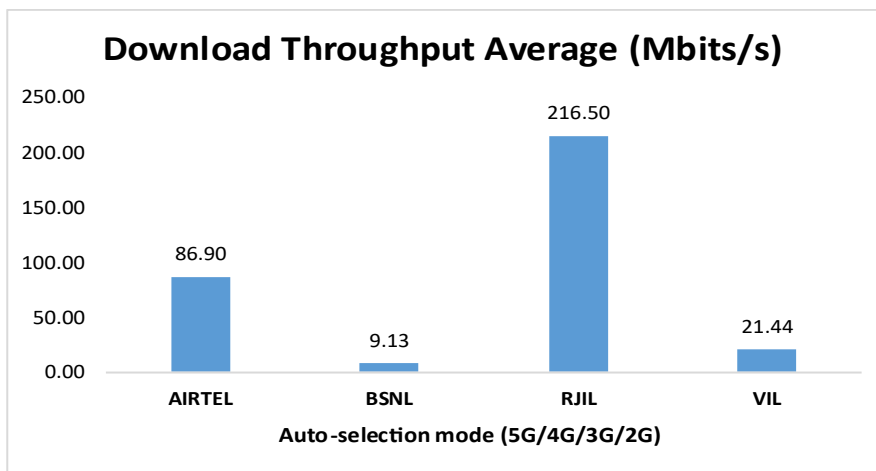
Figure 45: Download throughput.
