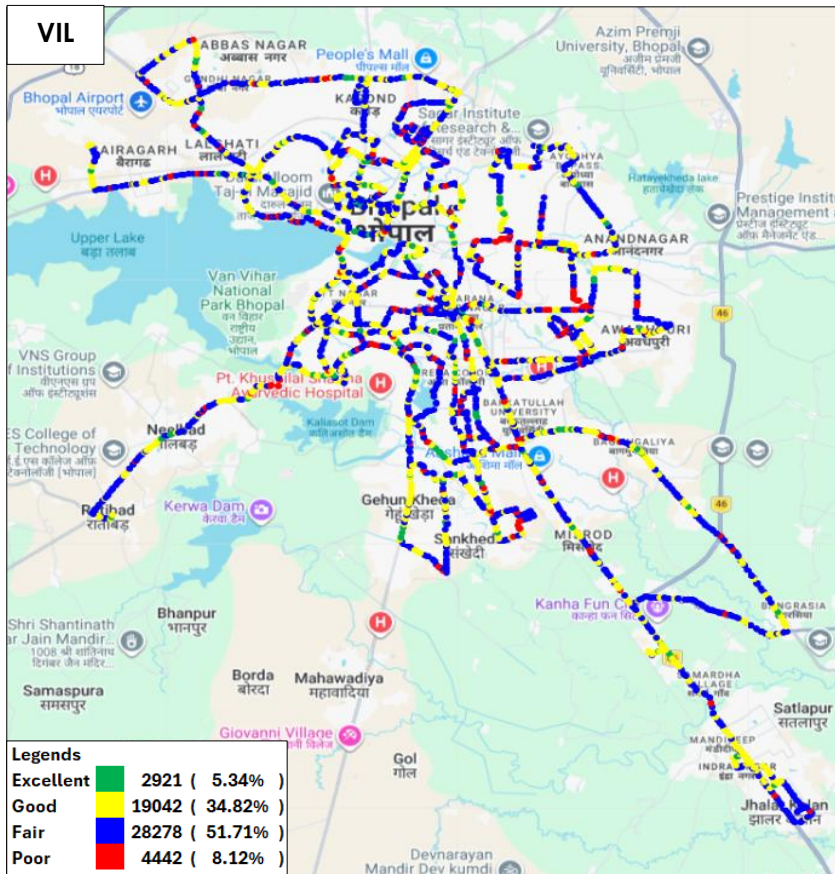
Figure-62: Signal strength auto-selection mode (5G/4G/3G/2G) data - VIL.
