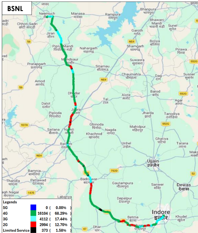
Figure-41: Serving technology plots in auto-selection mode (5G/4G/3G/2G) voice - BSNL.
