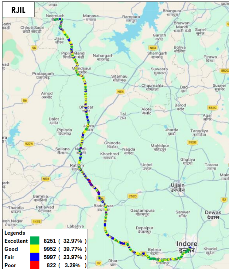
Figure-68: Signal strength auto-selection mode (5G/4G/3G/2G) voice - RJIL.
