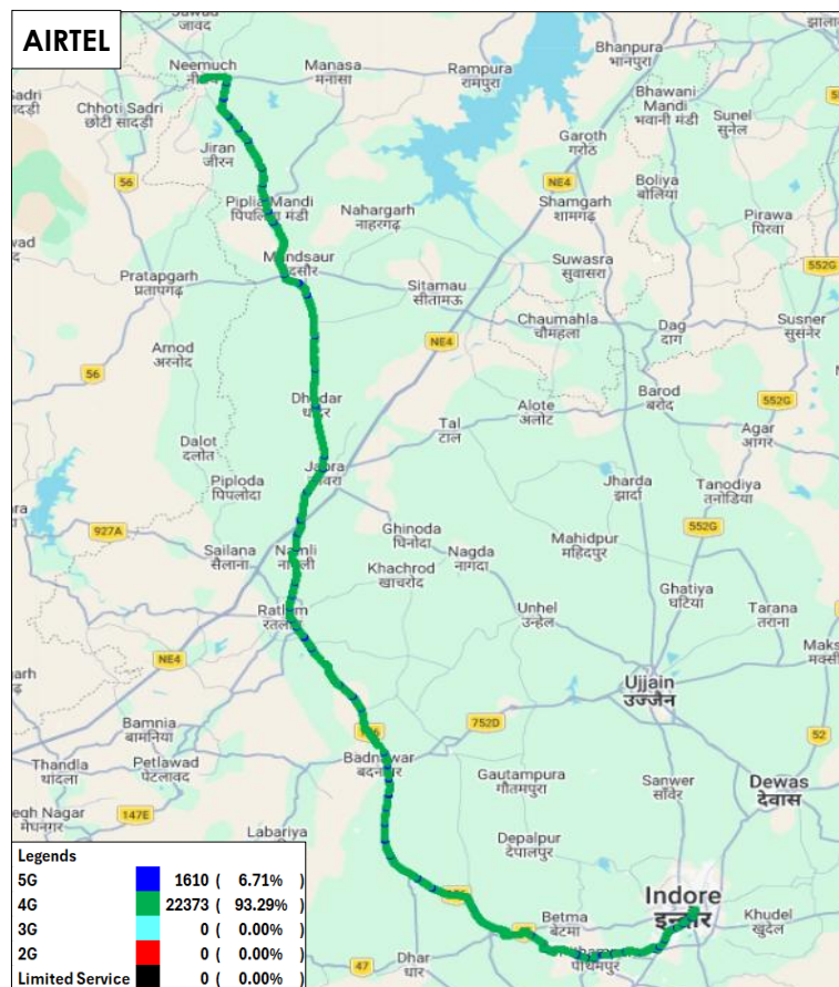
Figure-40: Serving technology plots in auto-selection mode (5G/4G/3G/2G) voice - AIRTEL.
