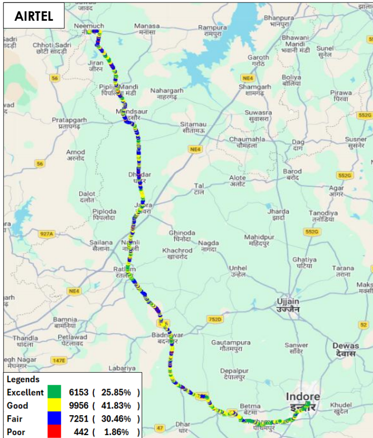
Figure-66: Signal strength auto-selection mode (5G/4G/3G/2G) voice - AIRTEL.
