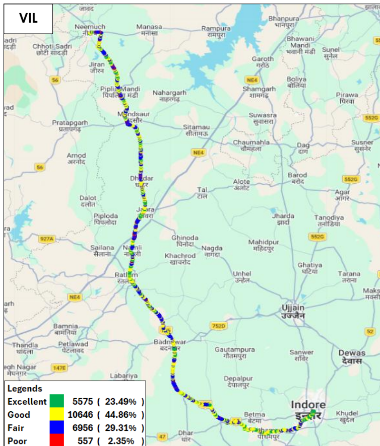
Figure-69: Signal strength auto-selection mode (5G/4G/3G/2G) voice - VIL.
