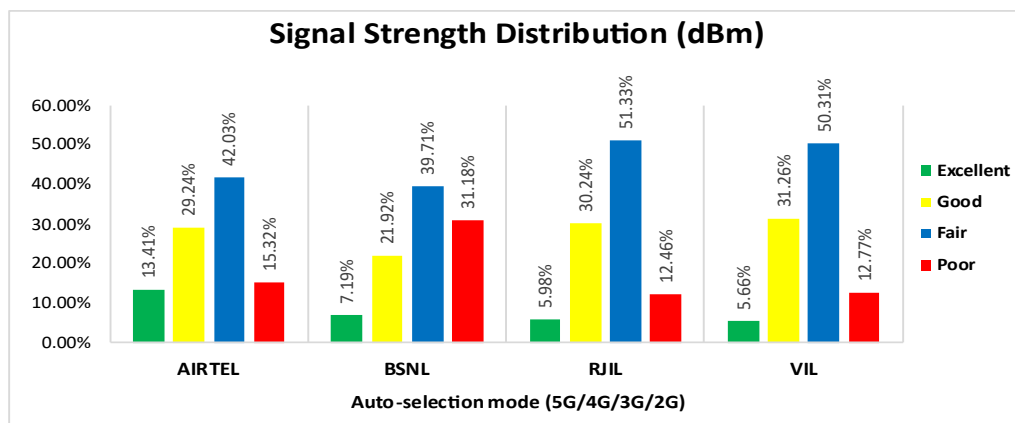
Figure-51: Signal strength distribution auto-selection mode (5G/4G/3G/2G) data.
