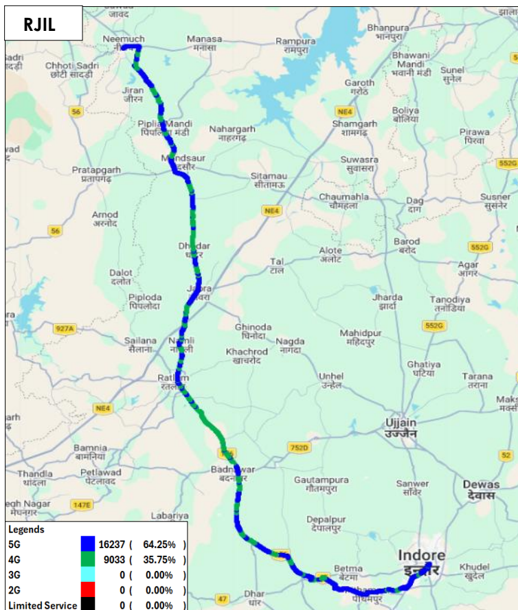
Figure-42: Serving technology plots in auto-selection mode (5G/4G/3G/2G) voice - RJIL.
