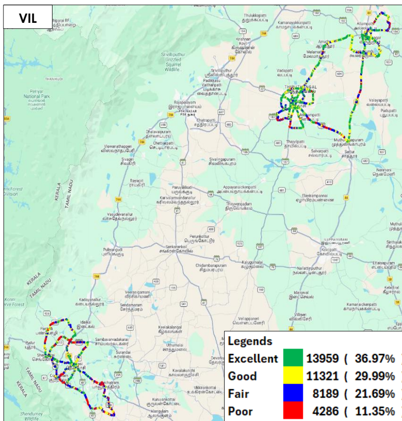
Figure-31: Signal strength 3G/2G network mode voice - VIL.
