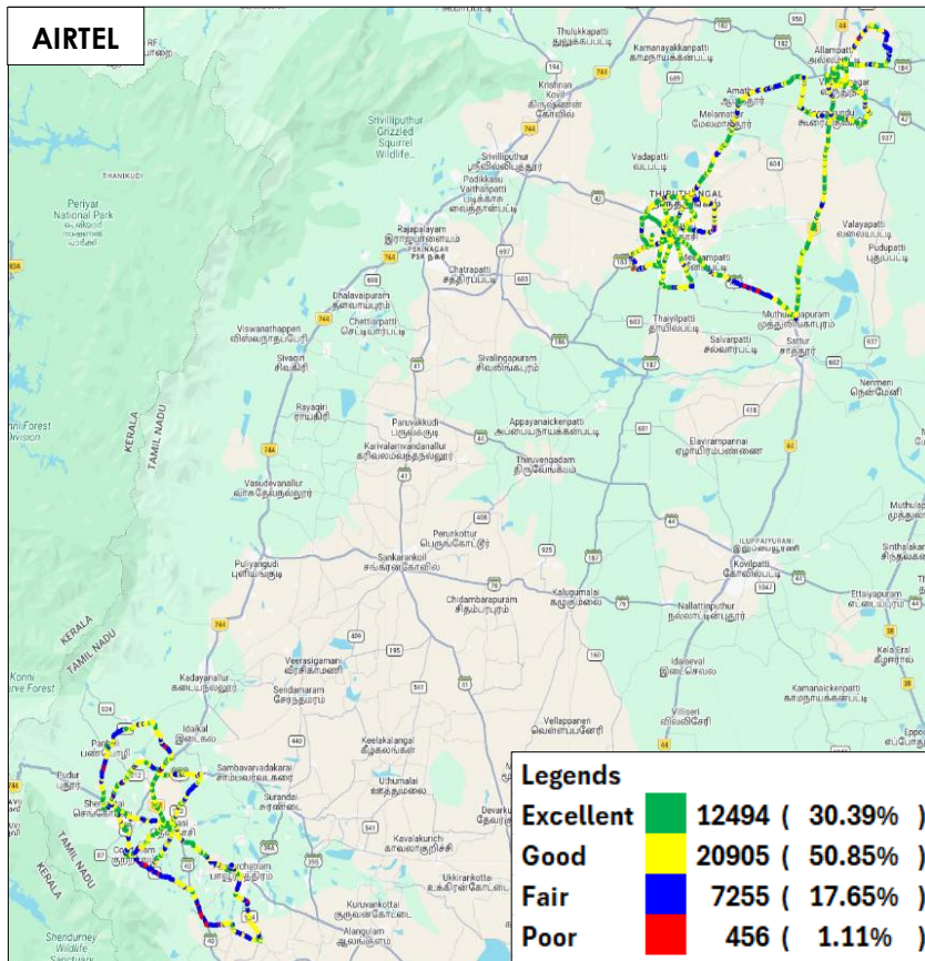
Figure-32: Signal strength auto-selection mode (5G/4G/3G/2G) voice - AIRTEL.
