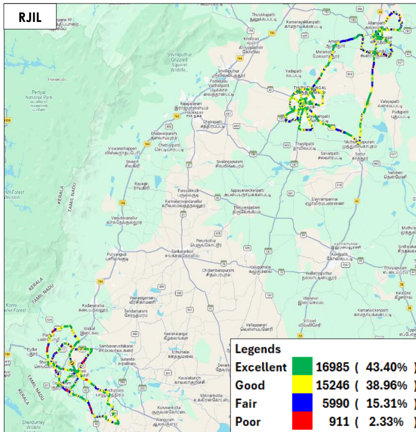
Figure-34: Signal strength auto-selection mode (5G/4G/3G/2G) voice - RJIL.
