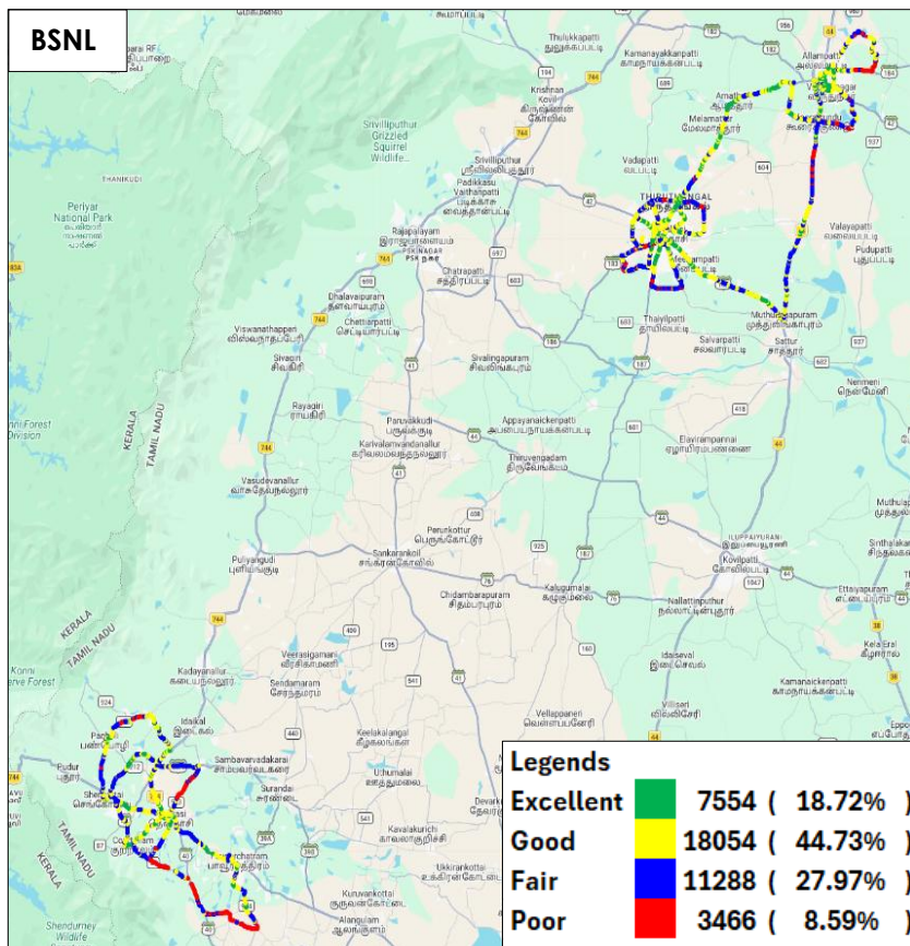
Figure-33: Signal strength auto-selection mode (5G/4G/3G/2G) voice - BSNL.
