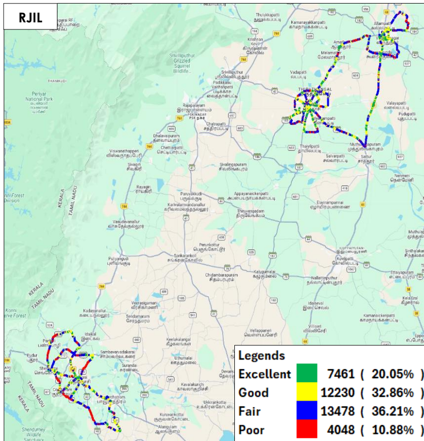
Figure-38: Signal strength auto-selection mode (5G/4G/3G/2G) data - RJIL.
