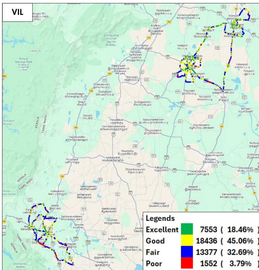
Figure-35: Signal strength auto-selection mode (5G/4G/3G/2G) voice - VIL.
